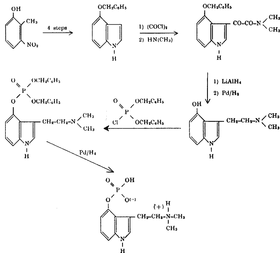
Fig. 4 - Synthesis of Psilocybin. Psilocybin
