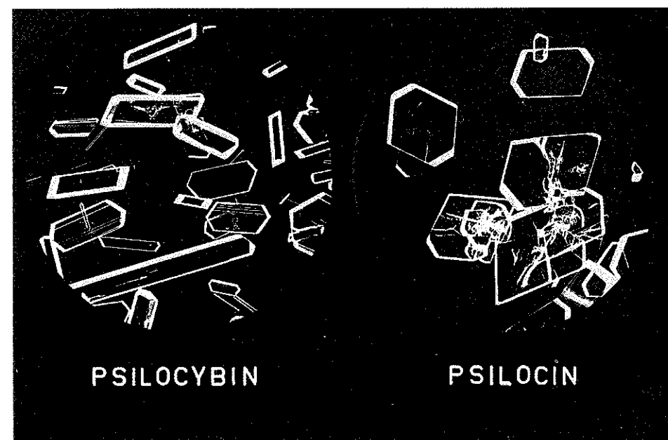
Fig. 3 - Psilocybin - Psilocin crystals.
